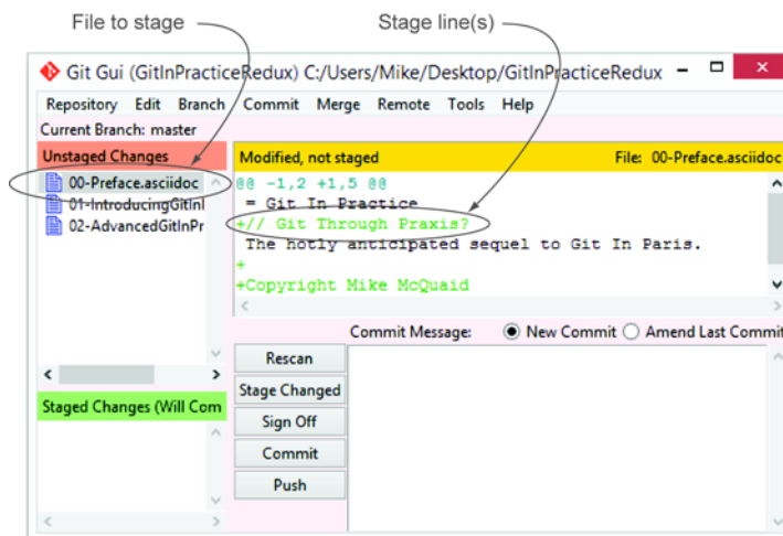
Figure 12.4 Git Gui on Windows 8.1
