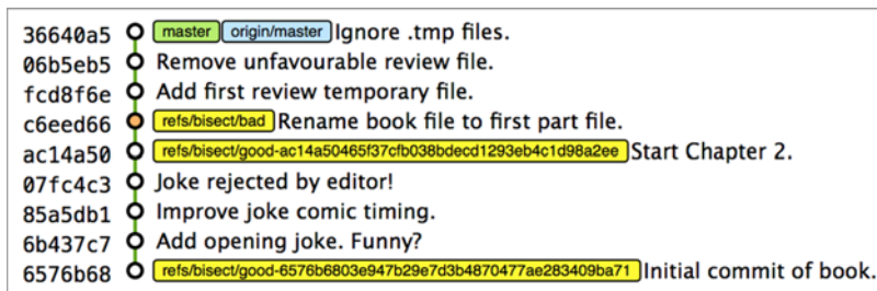
Figure 4.2 GitX bisect output before git bisect reset
