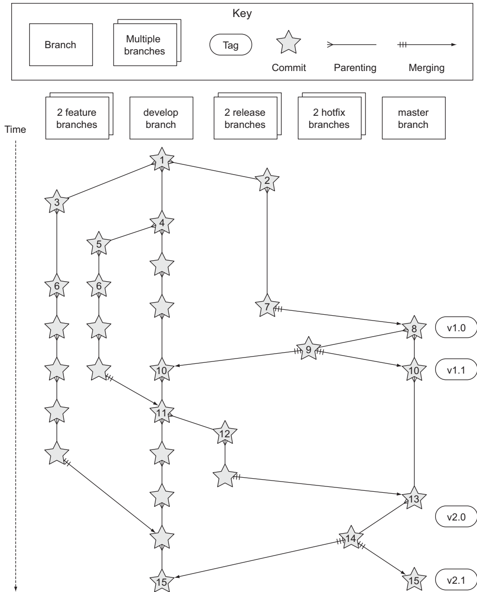
Figure 14.2 Git Flow
