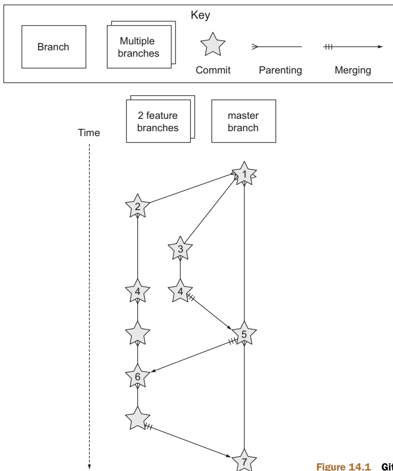
Figure 14.1 GitHub Flow
